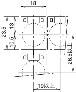
(AL-K6S 型)
